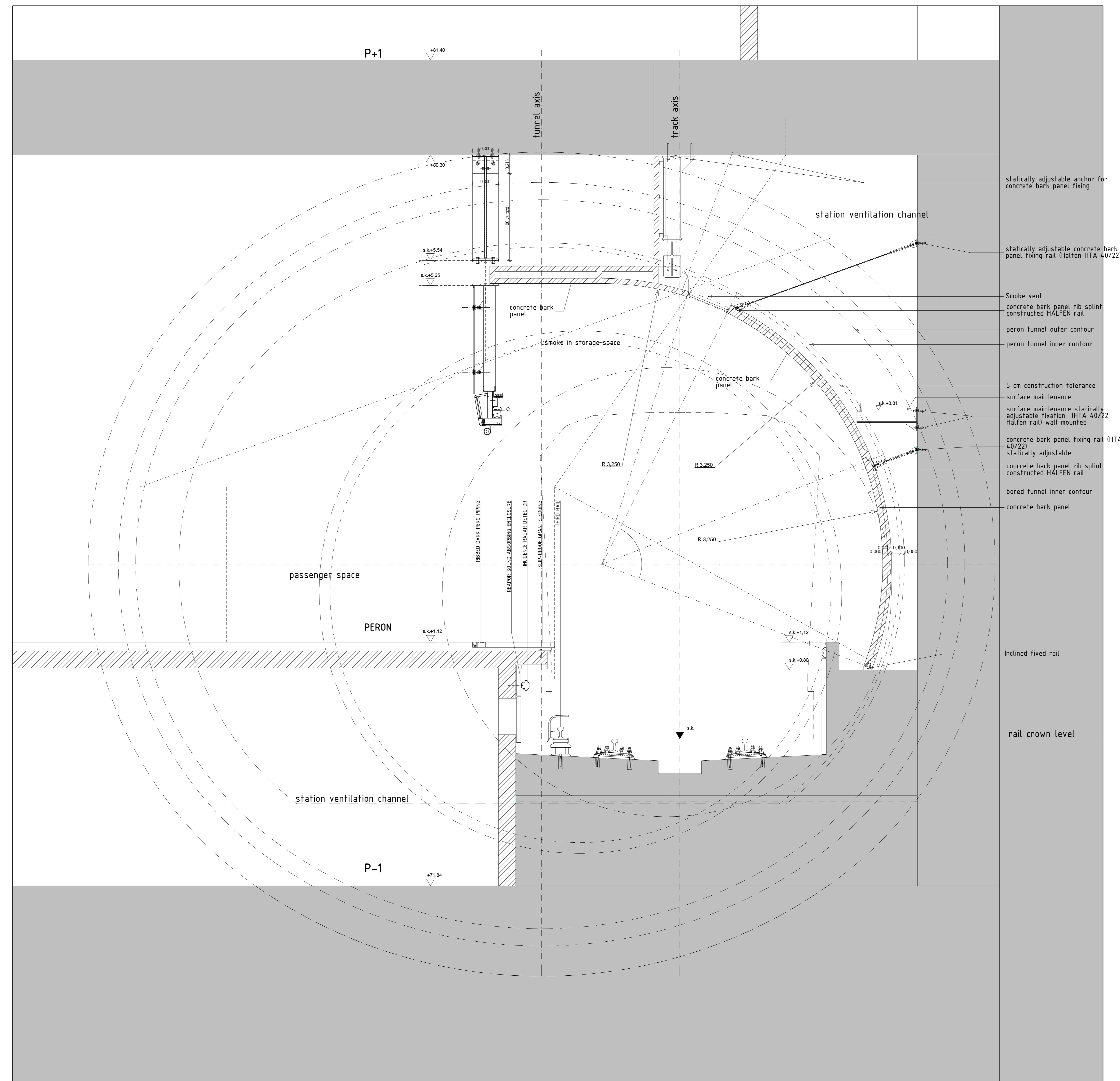
CONCRETE BARK PANEL IN STATION BOX detail 04.
