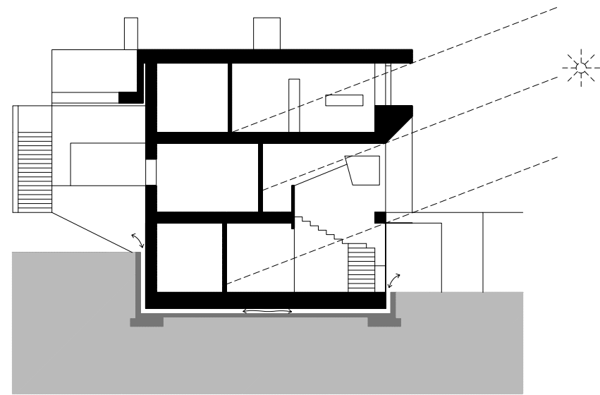
Cross Section
