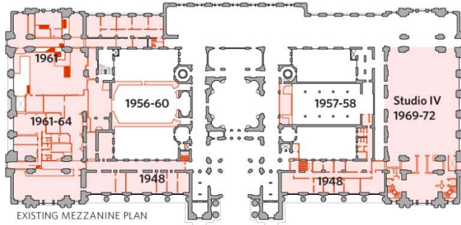
EXISTING MEZZANINE PLAN
